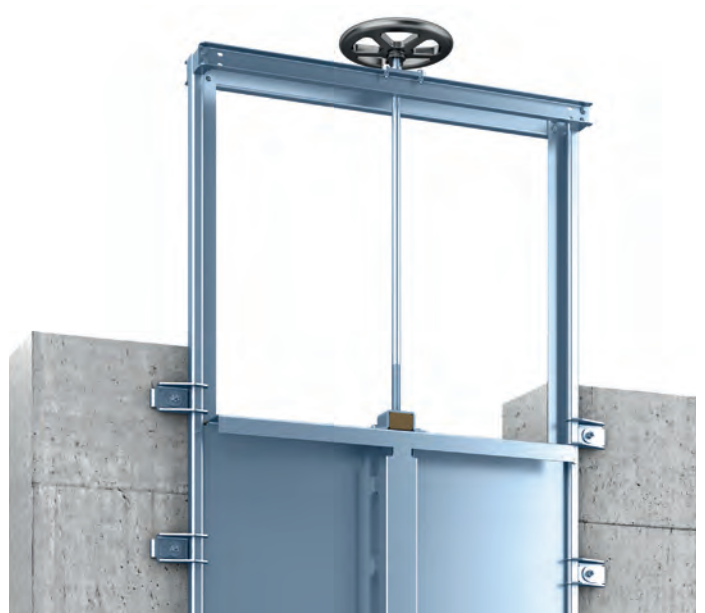
Passavant® Weir Sluice Gate
